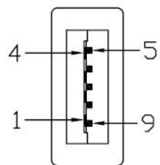
USB3.0 AM
