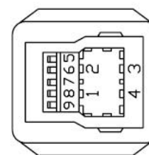
USB3.0 BM
